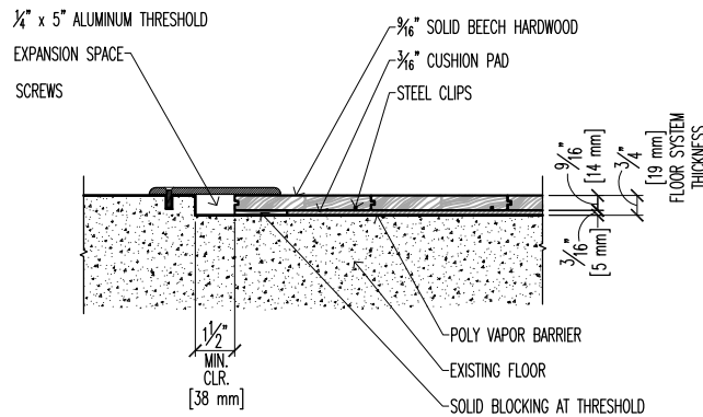
Studio Floor System - Threshold Detail
