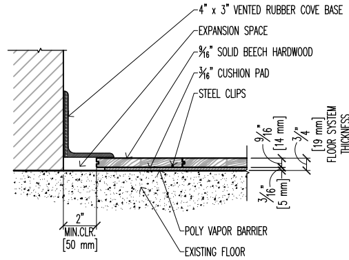
Studio Floor System - Wall Detail
